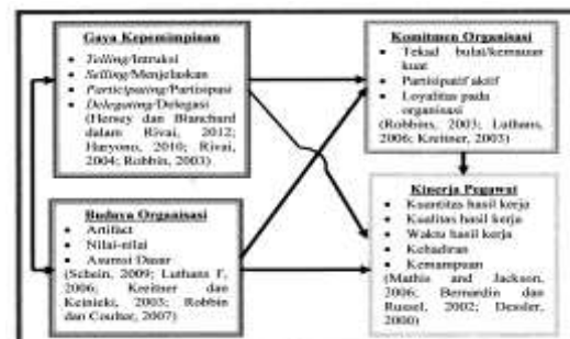
Gambar 1. Paradigma
