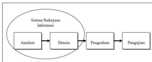
Gambar 1 Metode Waterfall [15]
